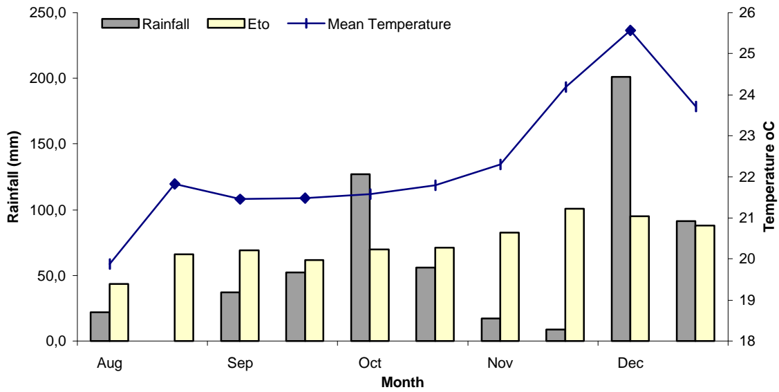
Figure 2. Rainfall, evapotranspiration, and mean temperatures reported by Fagundes (1999)
