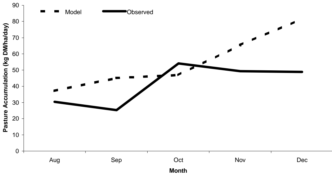
Figure 1. Herbage Accumulation (kg DM/ha/day) estimated by the Villa Nova Model and observed by Fagundes (1999)
